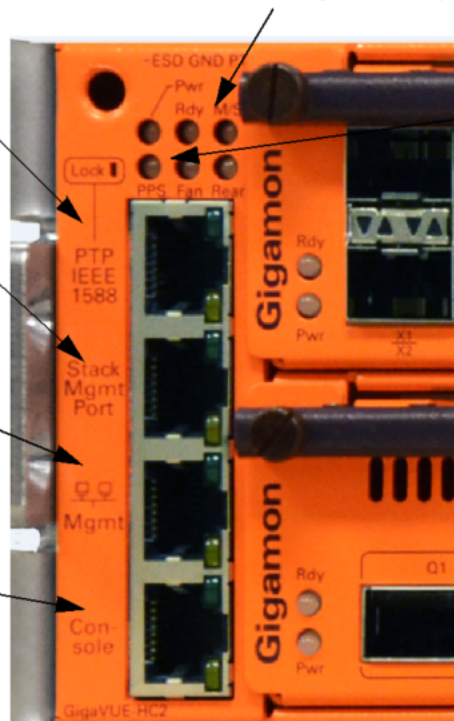
Figure 3 GigaVUE-HC2 Management Ports
